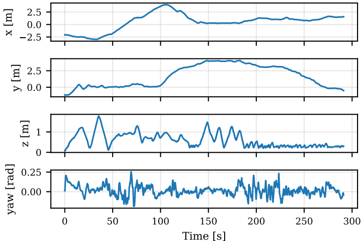
exp 6 - UAV 0 - Position
